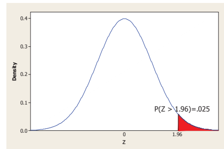
Fig 1d. N(0,1) : 2.5% right tail probability.
